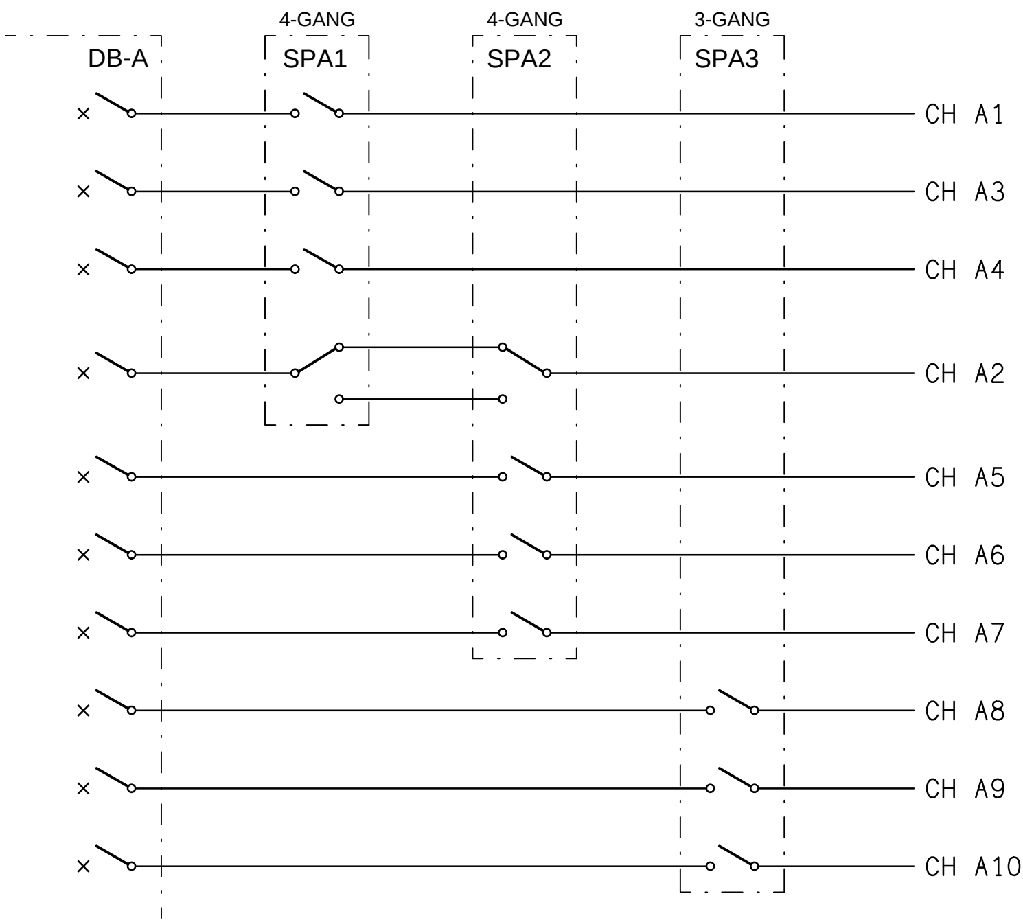
SCHEMATIC LIGHTING CONTROL NOT TO SCALE
